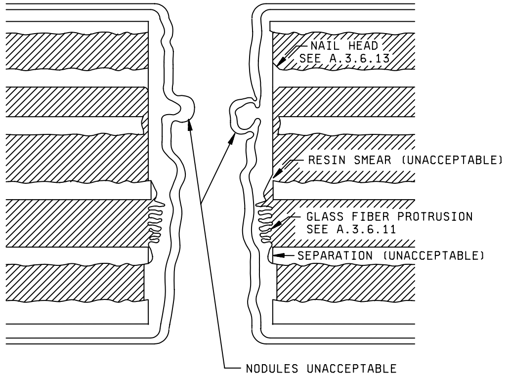
FIGURE A-16. Plated through hole deficiencies.
